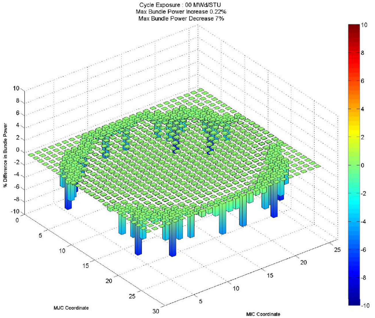
MIX Article Figure 3 – Change in Fuel Bundle Power with Reinserts at Oyster Creek Reactor
